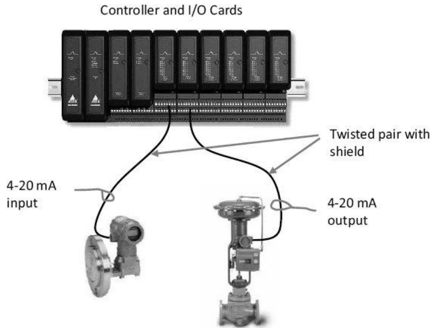
Figure 6-1. Wiring for Traditional Installation
