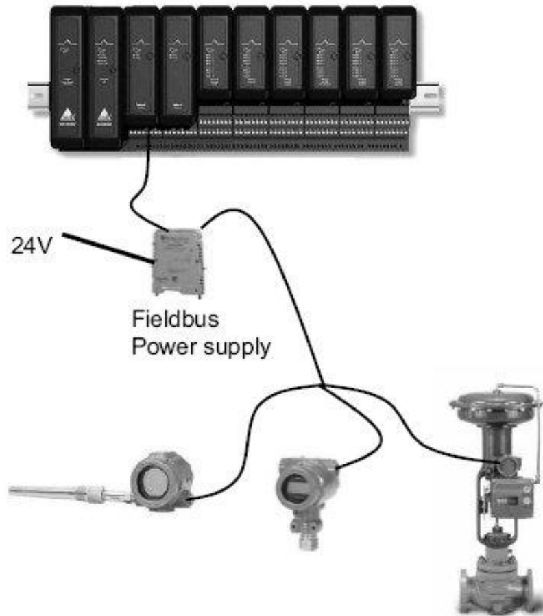
Figure 6-4. Foundation Fieldbus Segment
