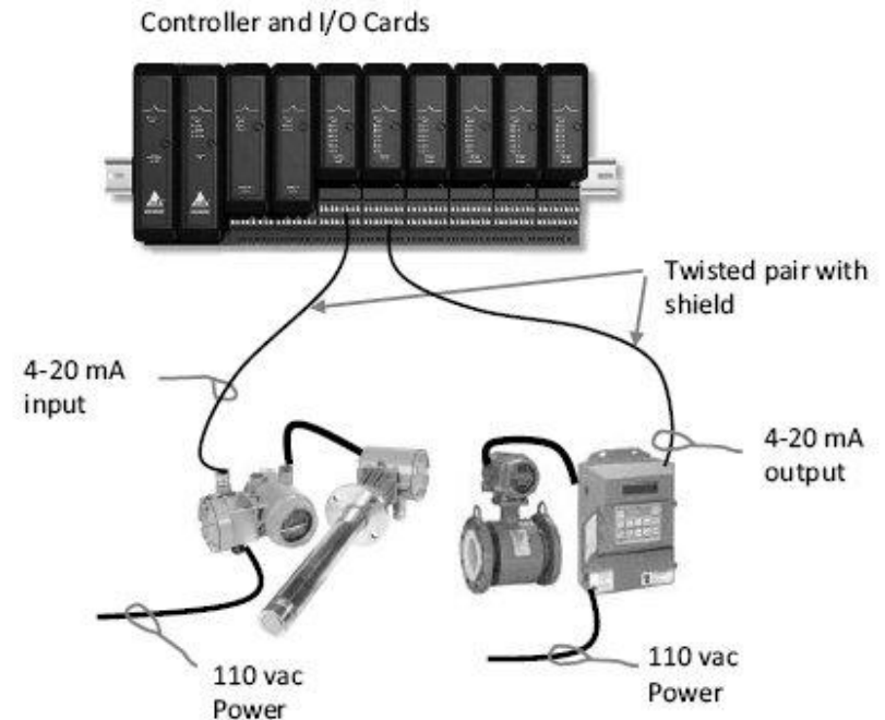
Figure 6-2. Wiring for Four-wire Transmitters
