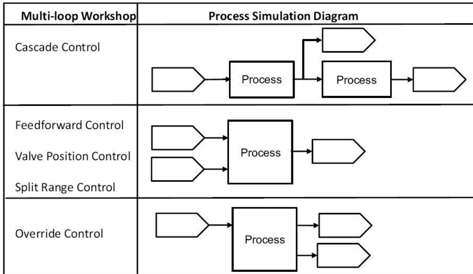
Figure 15-11. Simulation for Multi-loop Workshop
