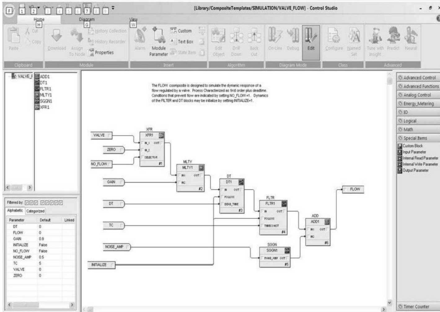
Figure 15-9. FLOW_VALVE Composite
