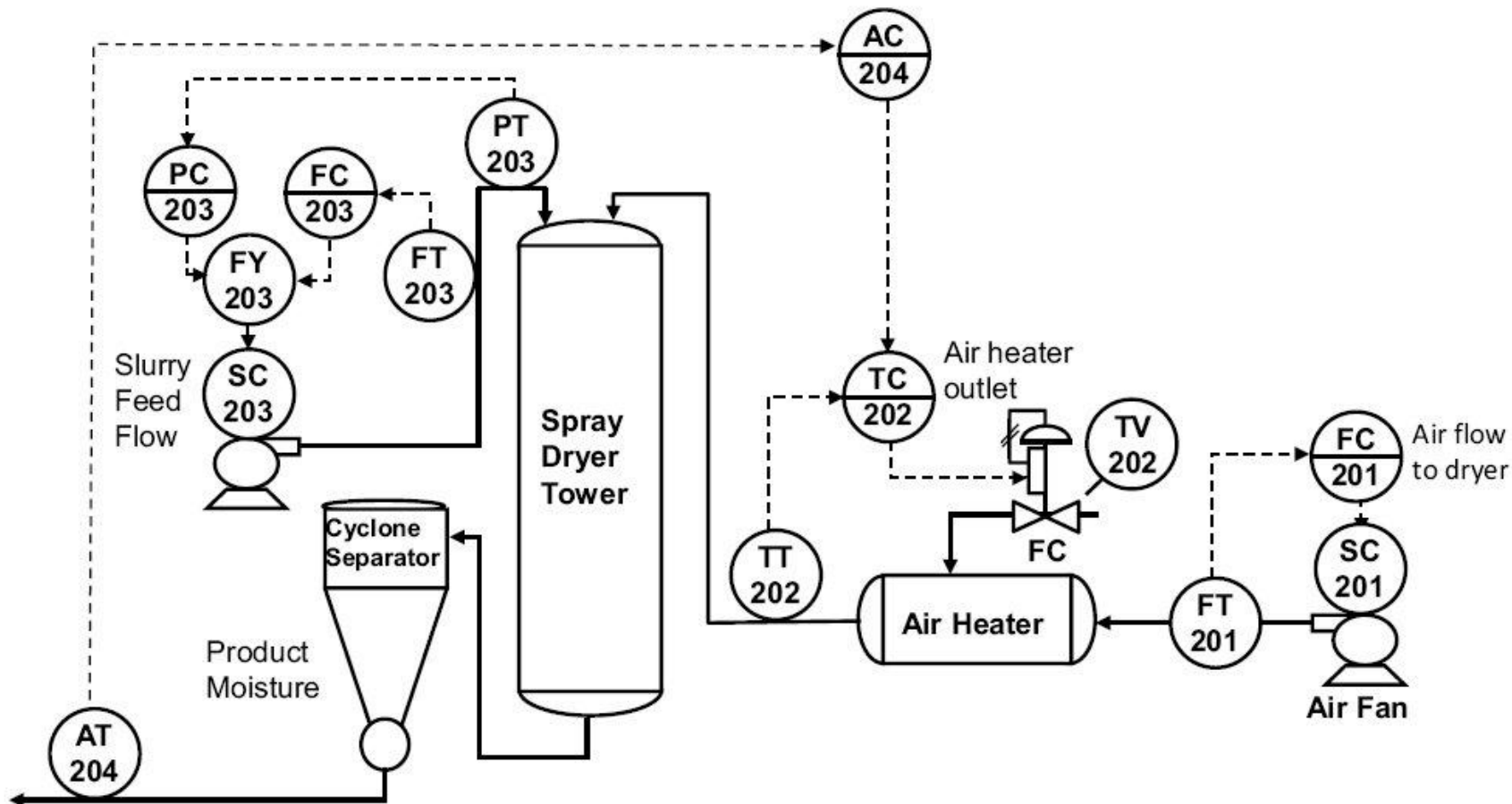
Figure 15-19. Spray Dryer Process
