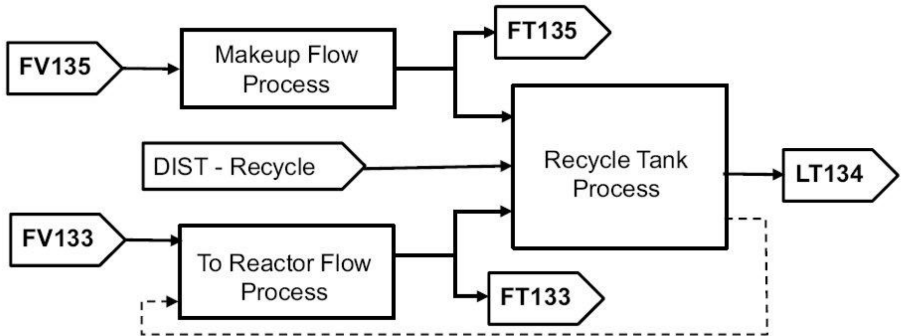
Figure 15-5. Diagram Showing Processes for Recycle Tank
