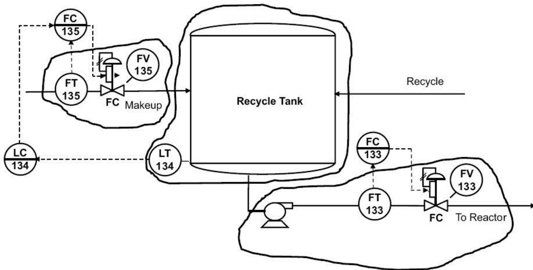
Figure 15-4. Breaking P&ID into Small Processes
