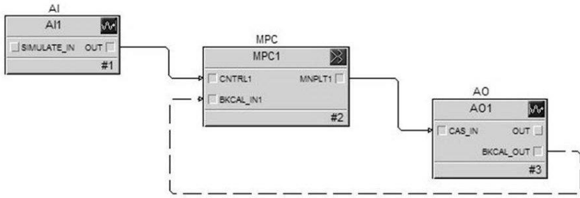
Figure 14-2. MPC Configuration for Single Loop
