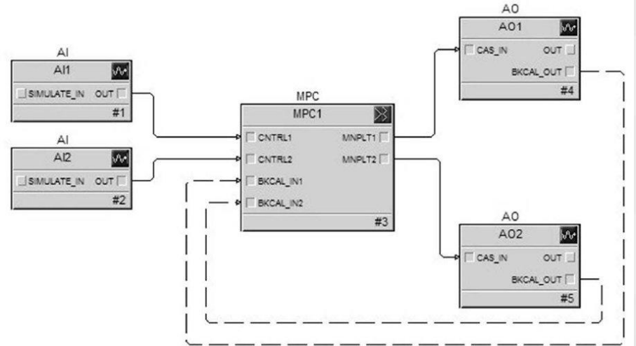
Figure 14-14. MPC Implementation for Interactive Process
